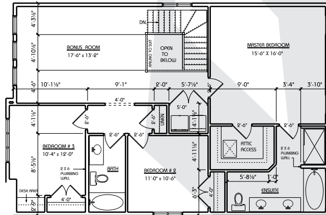
UPPER FLOOR PLAN 1236 SQ. FT.
